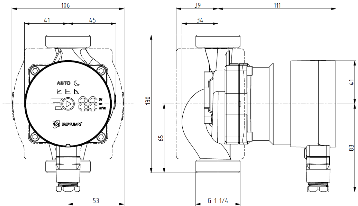
Dimension drawing
